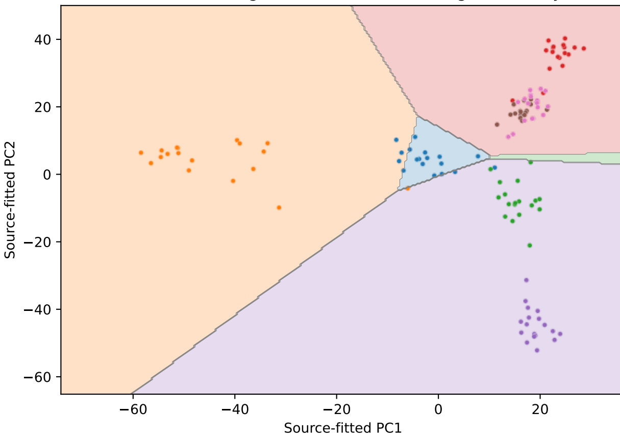
Original classifier on PCA plane; target points Slice/full-head agreement: 42.2% (not target accuracy)
