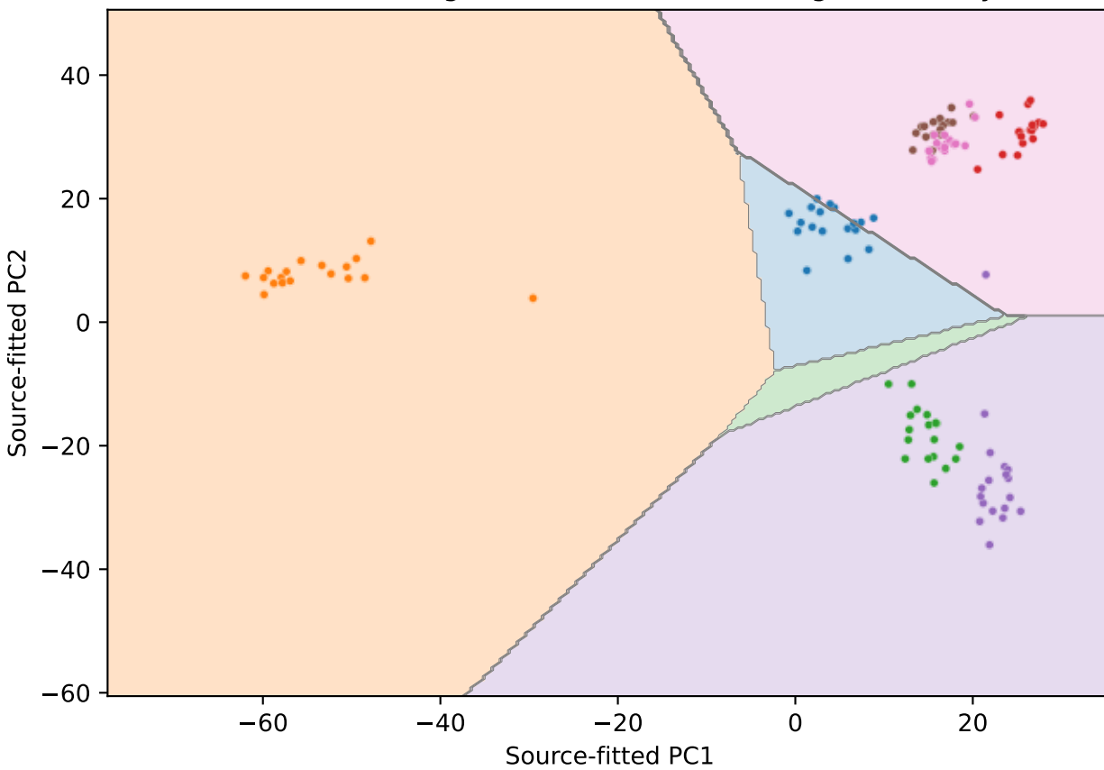
Original classifier on PCA plane; target points Slice/full-head agreement: 58.3% (not target accuracy)
