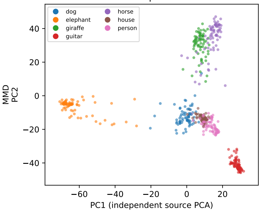
Class structure | variance 26.8%
