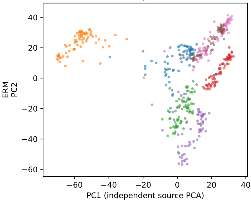
Class structure | variance 29.4%
