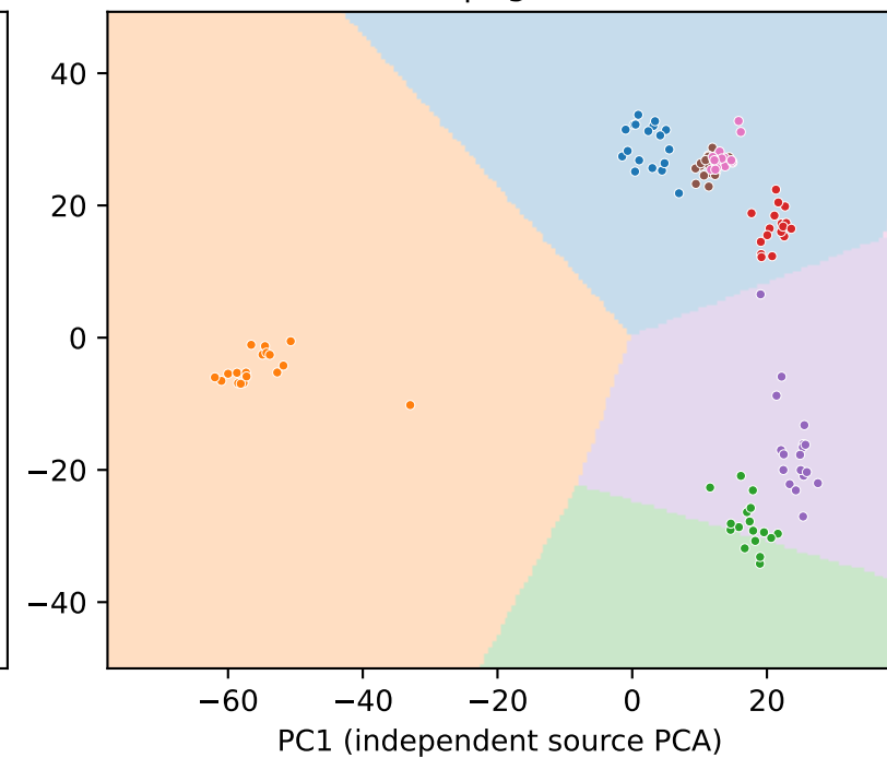
Classifier slice | agreement 45.7%
