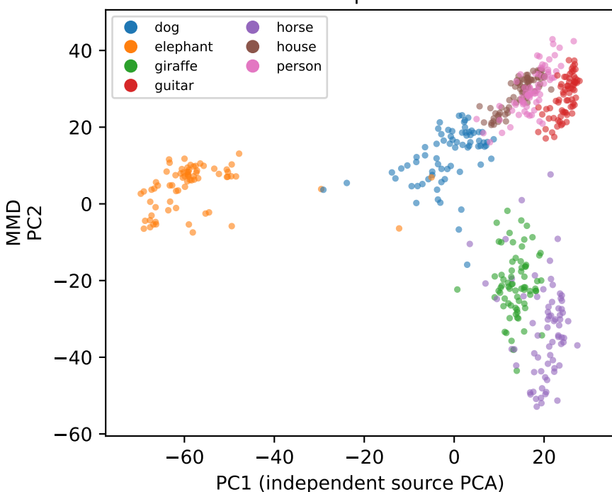
Class structure | variance 26.6%
