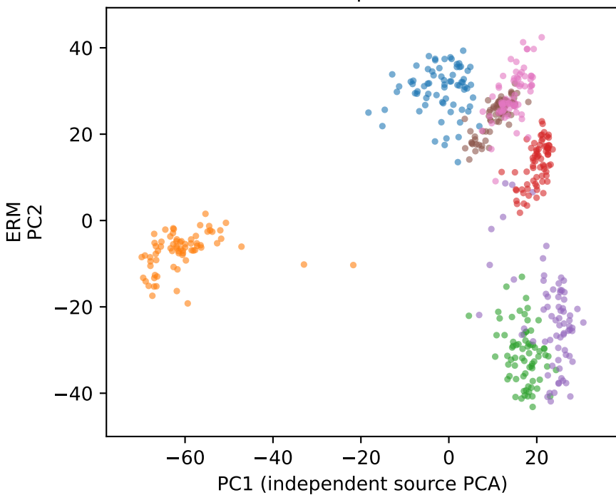
Class structure | variance 30.1%
