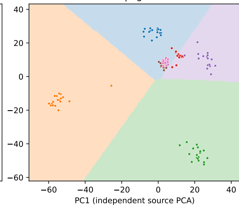
Classifier slice | agreement 58.3%
