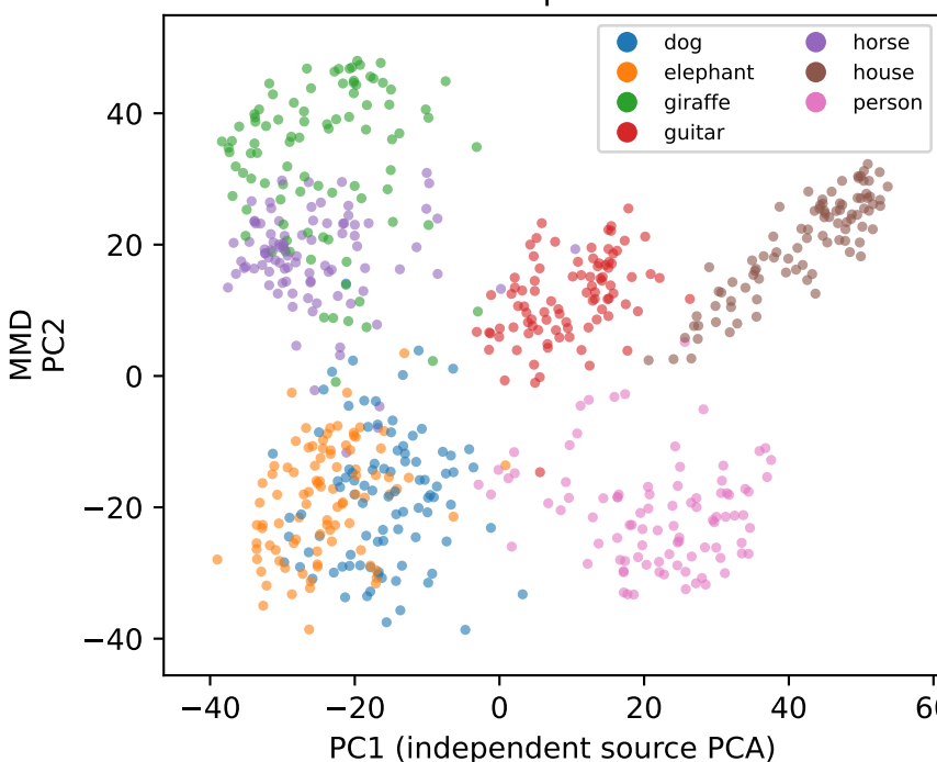
Class structure | variance 18.2%
