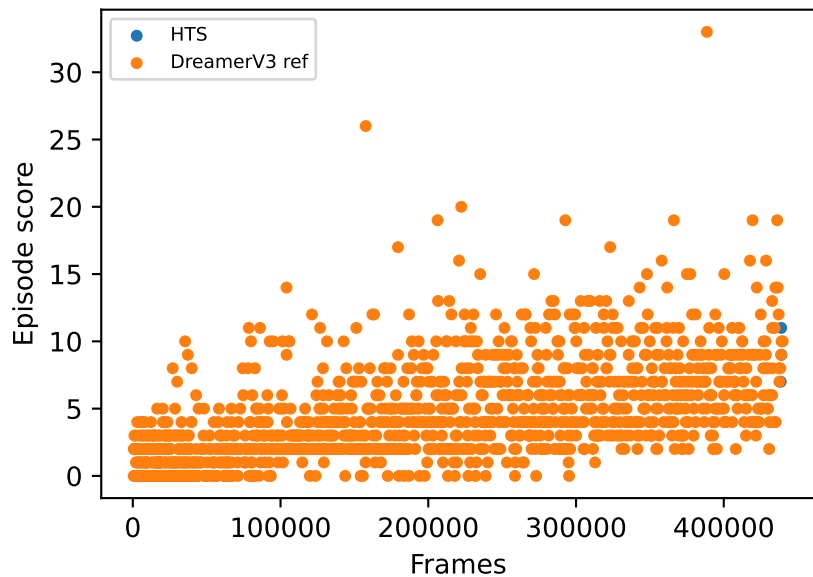
Breakout
