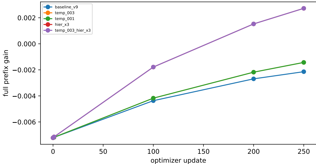
fig existing prefix gain trajectory v12
