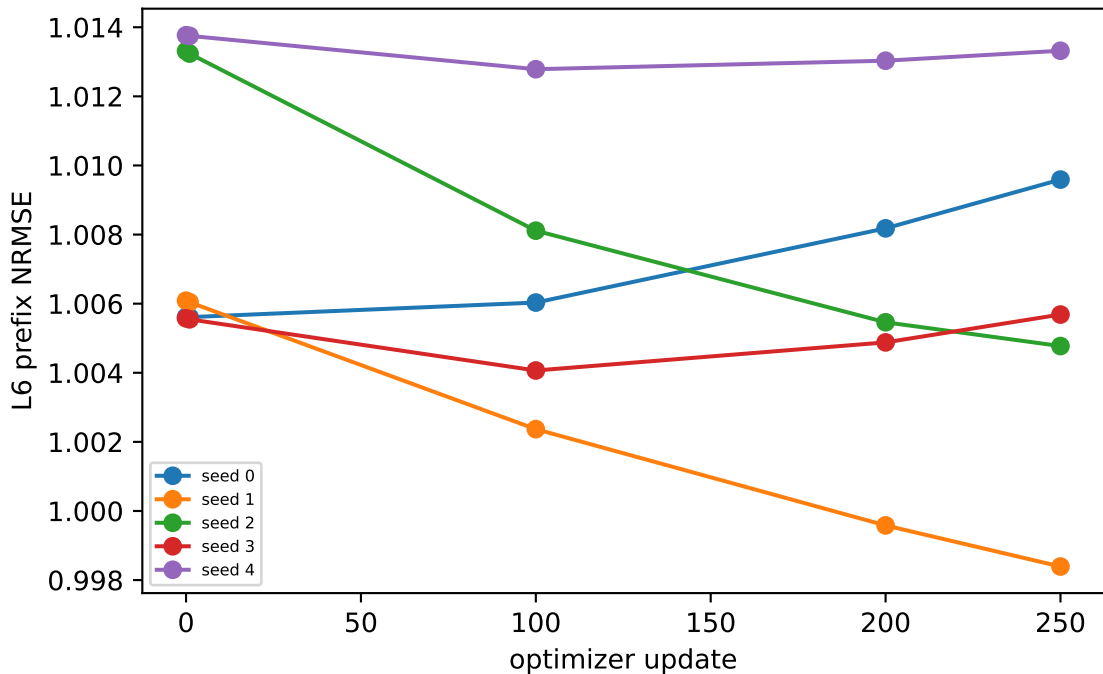
HTS prefix NRMSE by checkpoint V10
