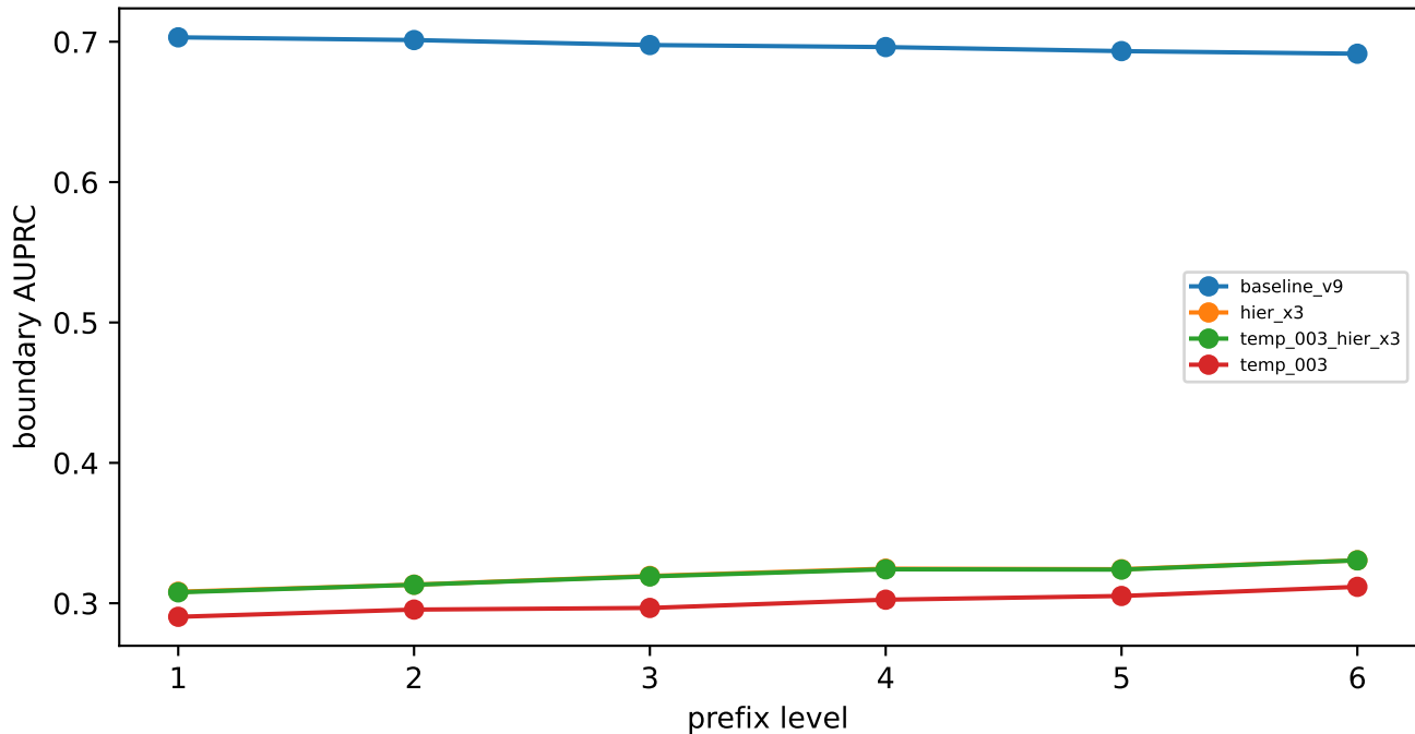
Boundary AUPRC by prefix V13
