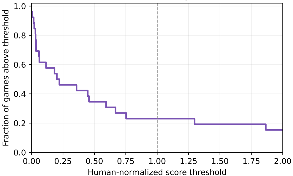
Human-level region
