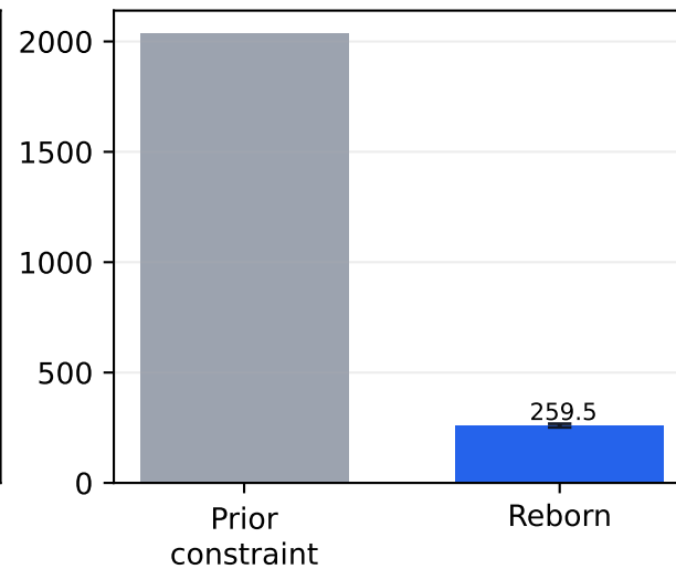
Frostbite
