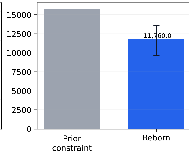
Road Runner
