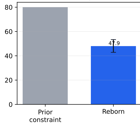
Boxing
