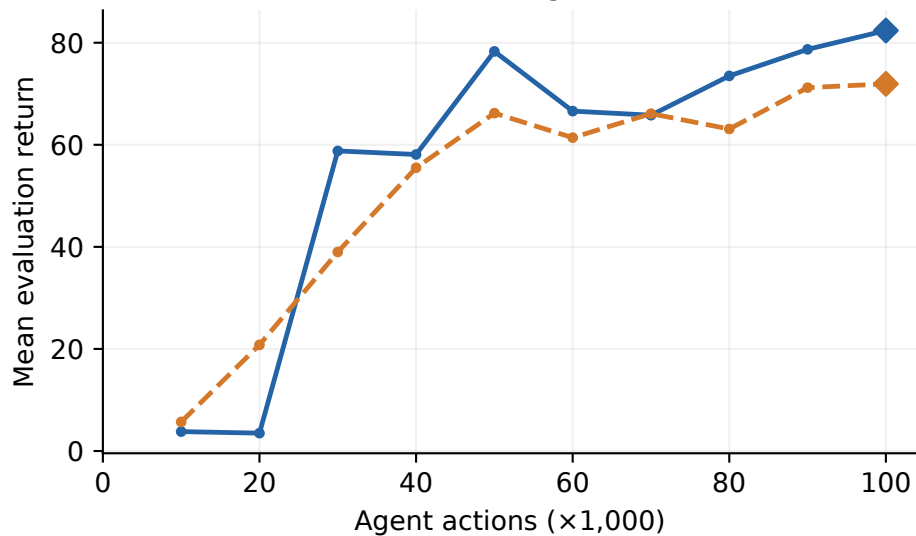
Frostbite
