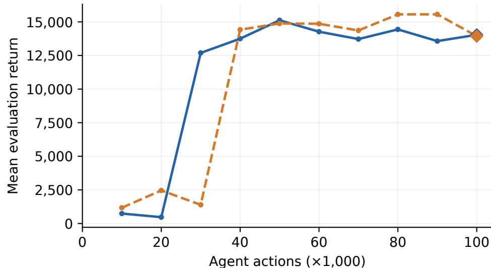
Road Runner
