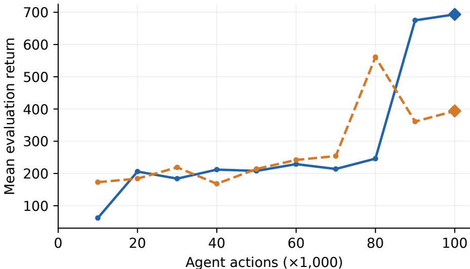
Frostbite
