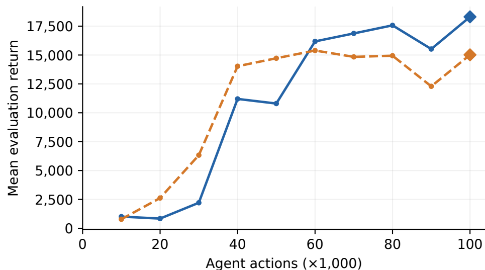
Road Runner
