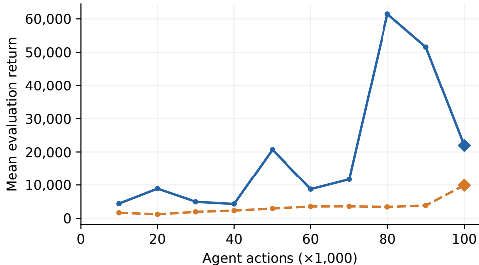
Road Runner
