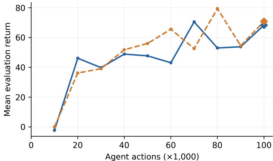
Frostbite
