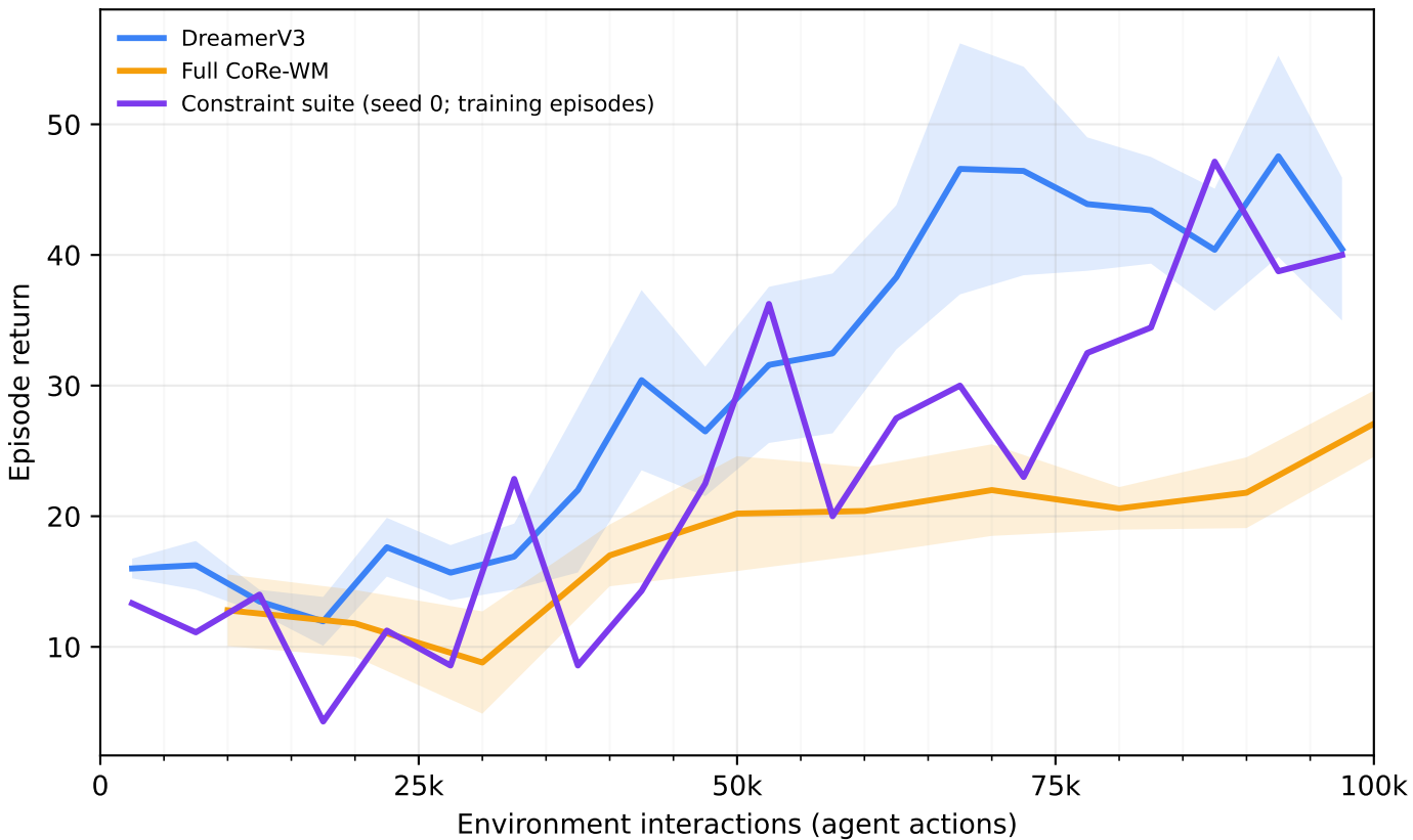
Bank Heist
