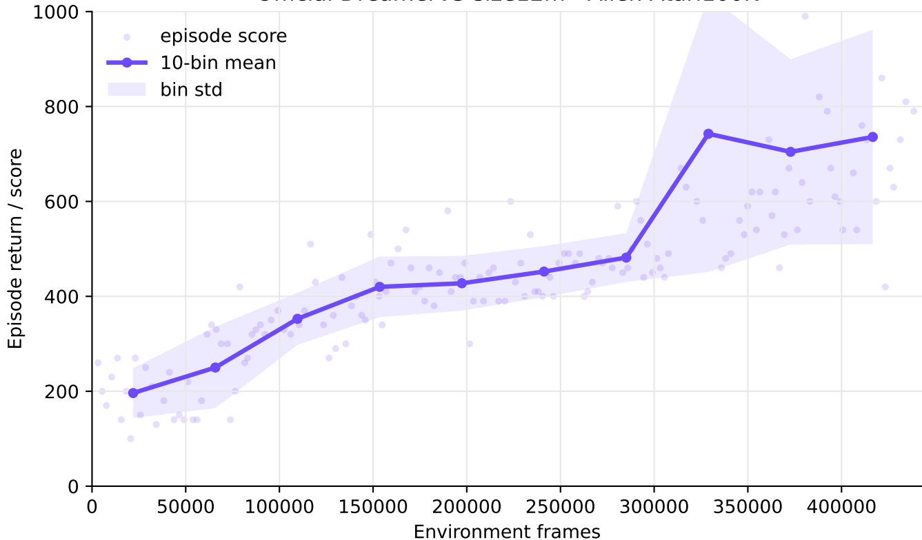
Official DreamerV3 size12m - Alien Atari100K
