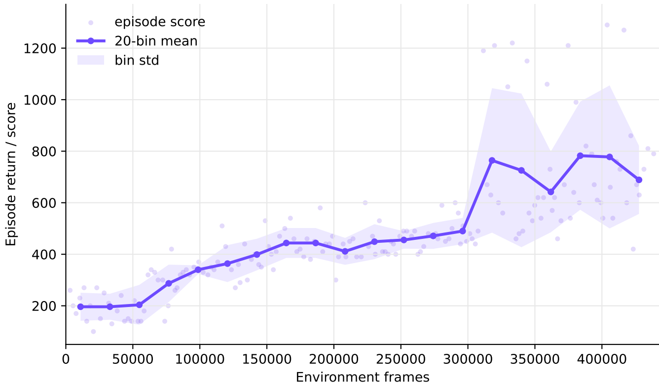
Official DreamerV3 size12m - Alien Atari100K
