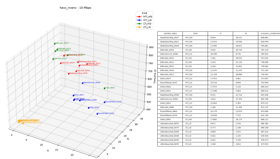
(g): hevc nvenc - bitrate: 10 Mbps
