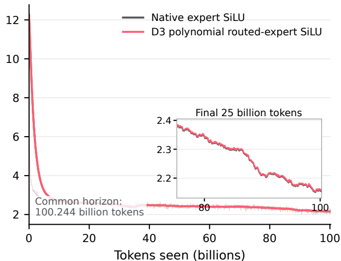
B4: expert SiLU in routed SwiGLU
