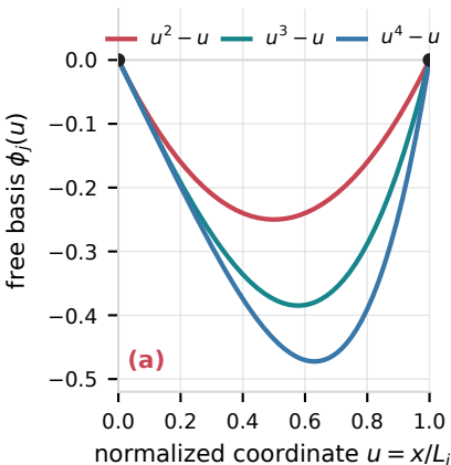
Endpoint-null basis
