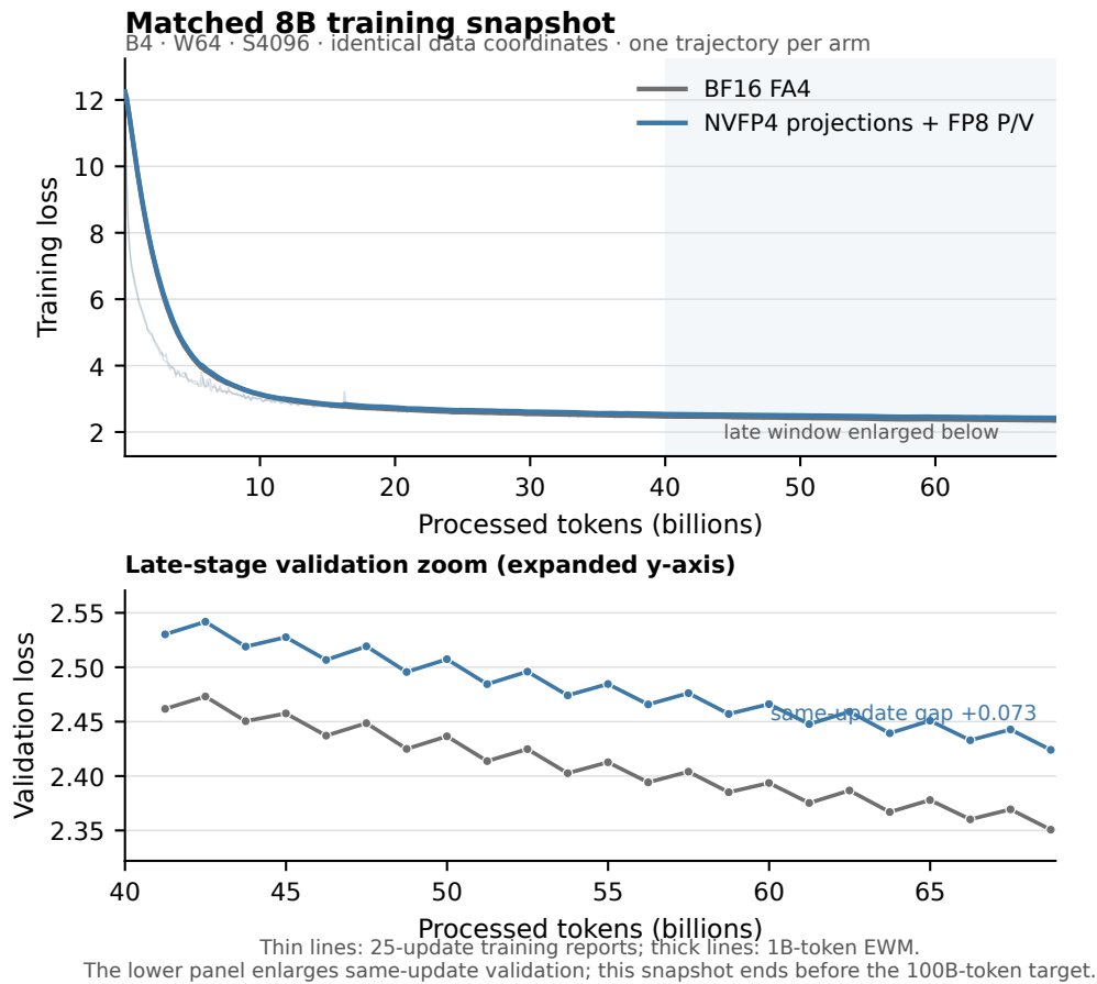
Figure 10: Token-aligned training and held-out validation for the matched B4 experiment through the reporting cutoff. The panel compares the BF16 control with the retained FP8-P/V route; the lower panel magnifies same-update validation from 40 billion tokens onward with an expanded vertical axis. Each curve is one trajectory, so the plot provides no uncertainty estimate.
