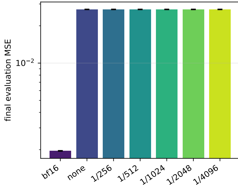
Generalization floor
