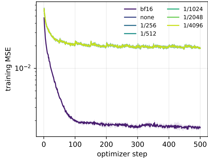
Teacher/student regression
