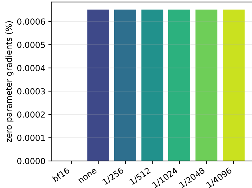
Last 20 steps
