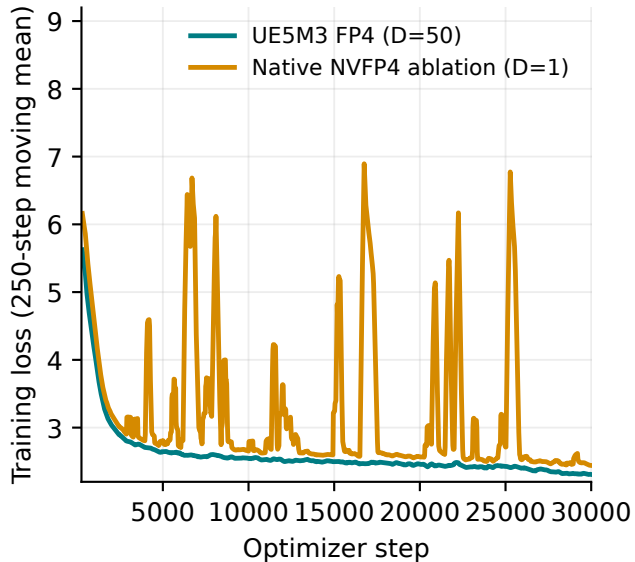
Training-loss trajectory
