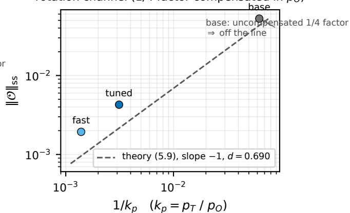
rotation channel (1/4 factor compensated in p_O )
