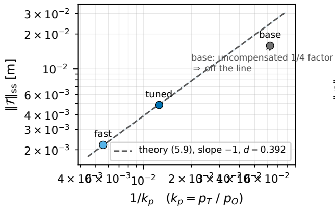
translation channel (empirical slope -0.98 vs -1 )
