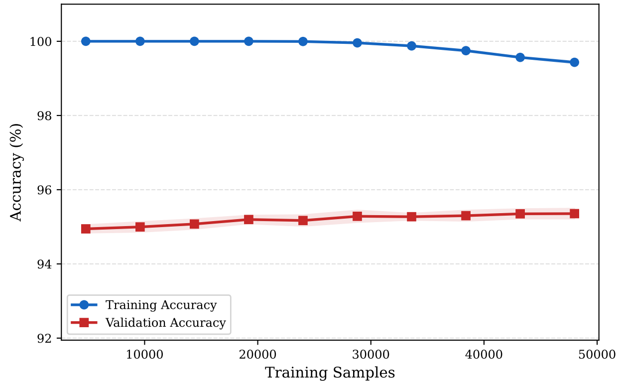
(a) Accuracy vs. Training Set Size
