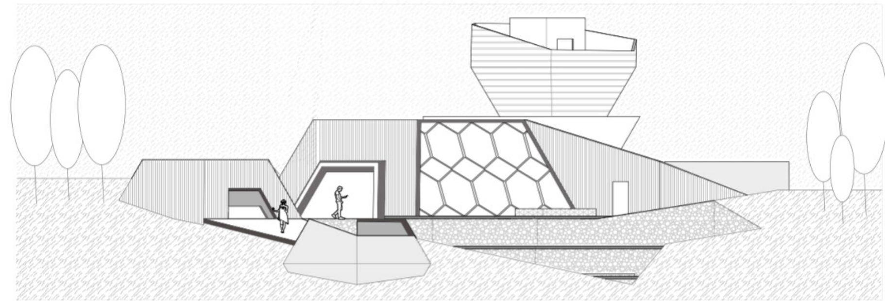
ELEVATION | EAST 1/4" = 1'
