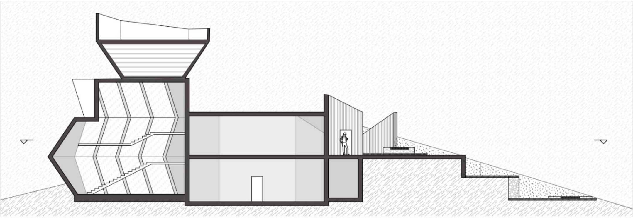
SECTION | NORTH-SOUTH 1/4" = 1'
