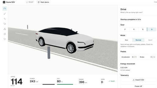
(a) Drive at 114 km/h: the dashboard strip under the stage shows speed, power, SOC, range and gear, all from bus frames.
