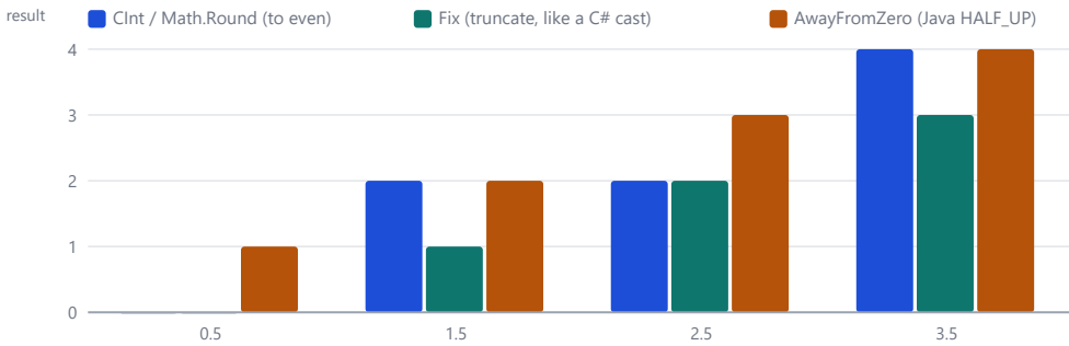
measured: L06.VbSemantics output in 4.6 · C# (int) and Java HALF_UP columns named by the rule they share
