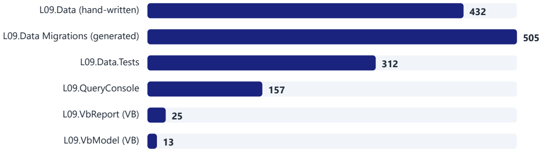
non-blank, non-comment lines · measured from the sample files when this PDF was built
