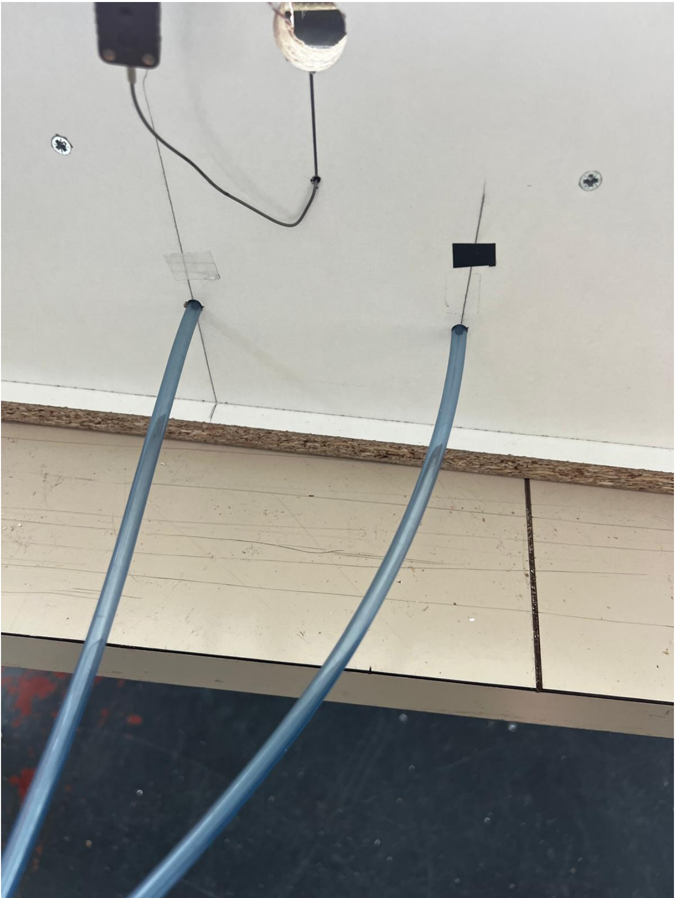
Figure 4: Pressure port tubes through the tunnel wall
