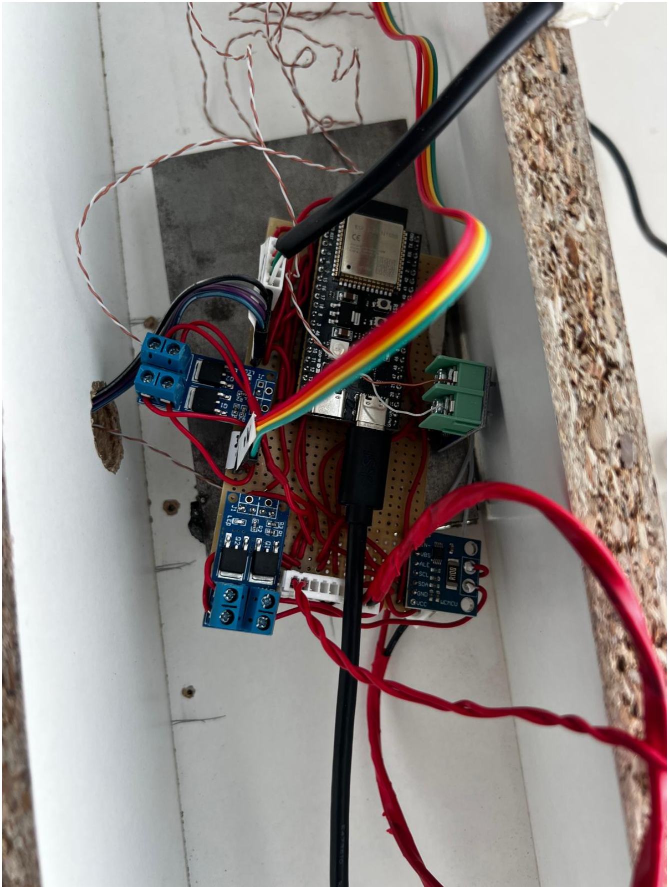
Figure 6: Dev board fully installed and wired
