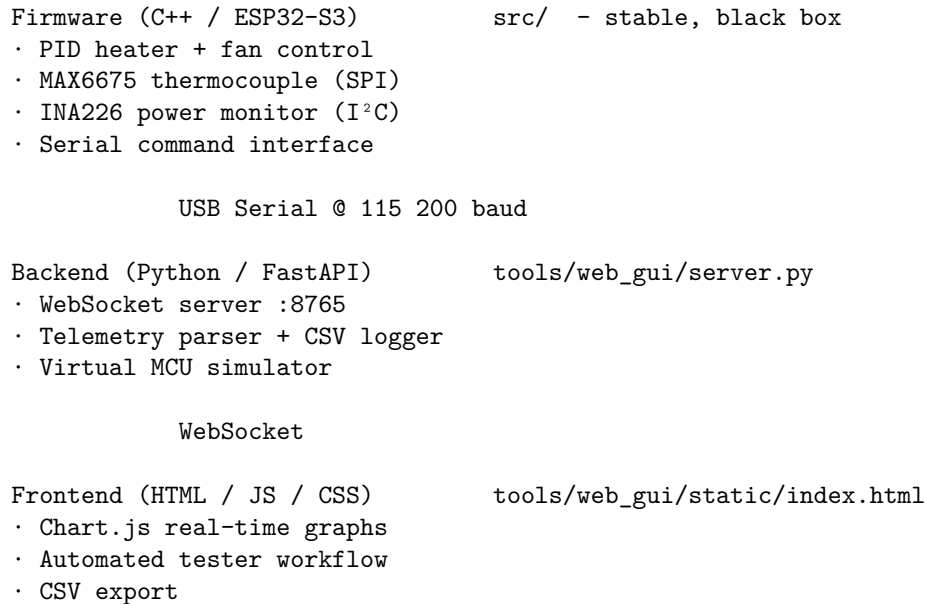
Figure 3.1 - Three-tier architecture. The only contracts between tiers are the serial command/telemetry protocol (firmware ↔ backend) and the WebSocket message set (backend ↔ frontend).
