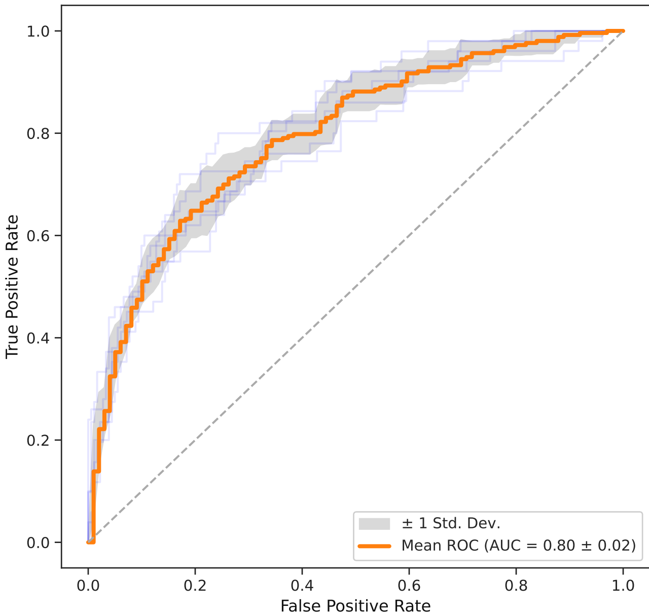
ROC Curve Analysis - Training Folds
