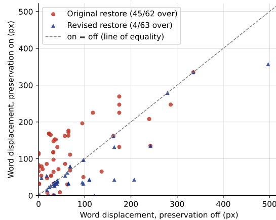
Fig. 4. Displacement of the anchor word with preservation ON against its displacement OFF, one point per complete pair (62 original, 63 revised). Points above the line of equality mean the restore moved the word further than the reflow alone (by more than 1 px in 45 pairs with the original restore, circles, and 4 with the revised one, triangles). The two versions were captured in separate runs.
