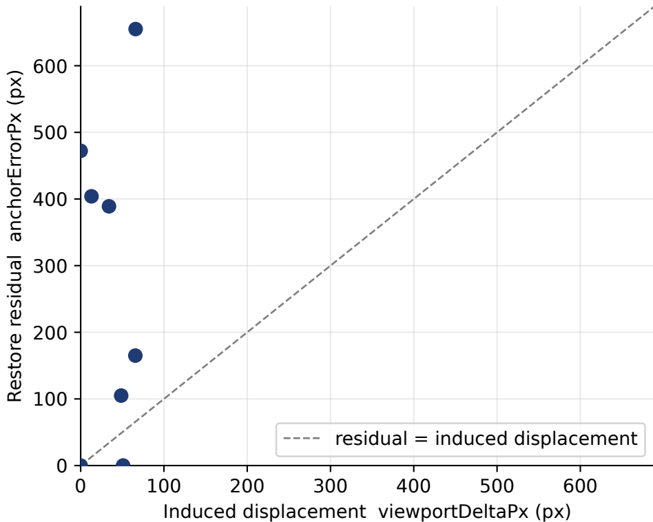
Semantic-restart over-repositions on small reflows
