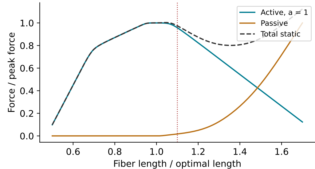
Original force-length curves
