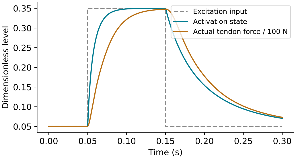
Held length: force is a response
