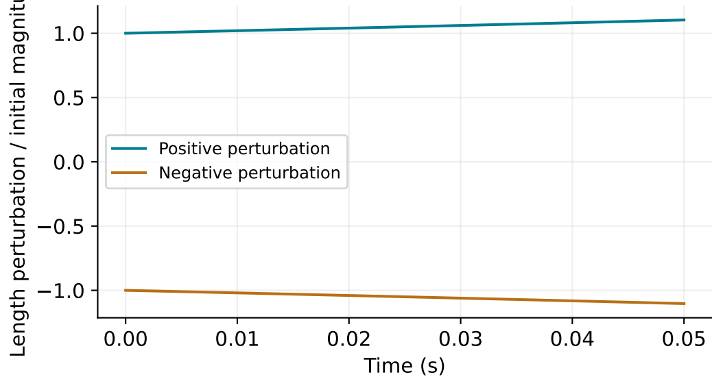
Fixed force: descending instability retained
