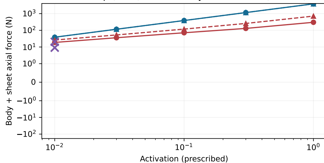
Direct cap (solid) / whole-body virtual force (dashed)
