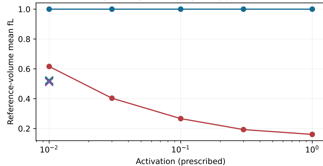
Operating force-length suppression
