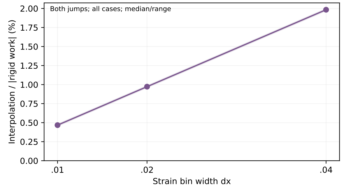
Upwind interpolation adds positive work
