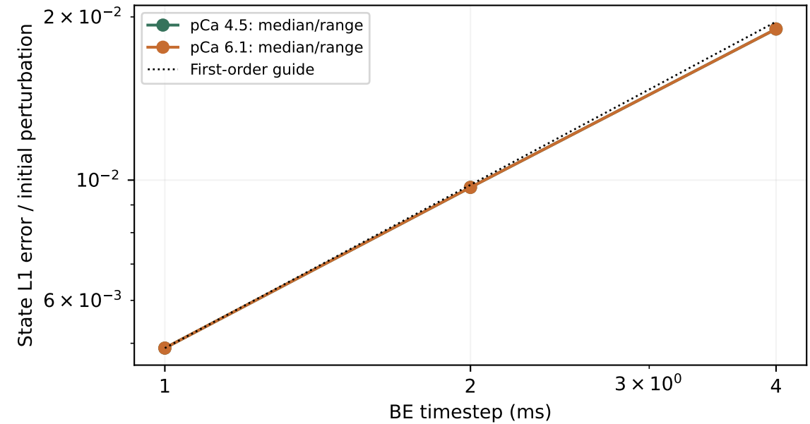
Time error against independent bin dynamics
