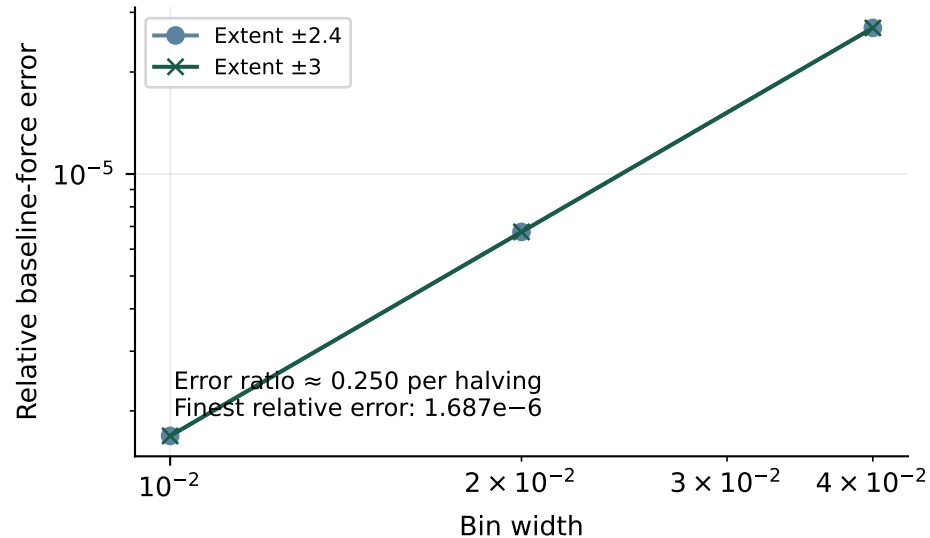
Spatial equilibrium error against quadrature
