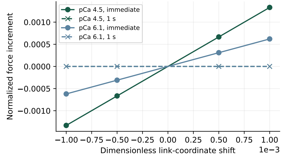
Immediate and relaxed increments differ
