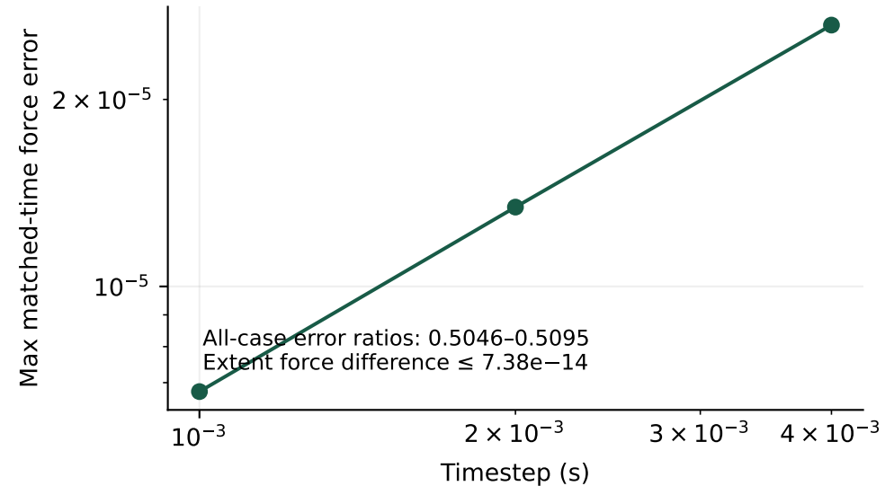
Temporal error against exact finite generator
