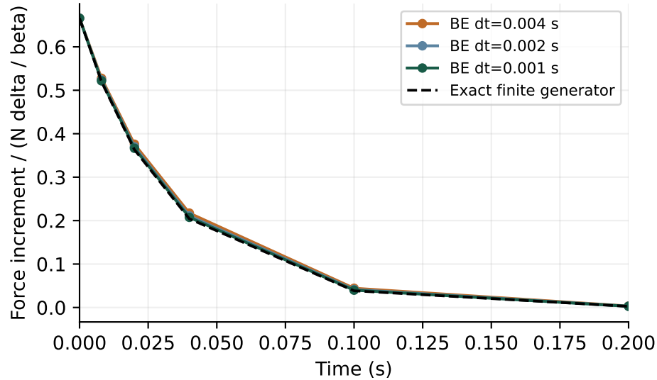
Matched-time relaxation after +0.001 shift
