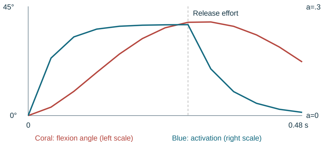
Coupled tissue / tendon / hinge: computed pulse
