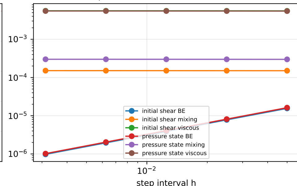
Separate accumulated discrete losses
