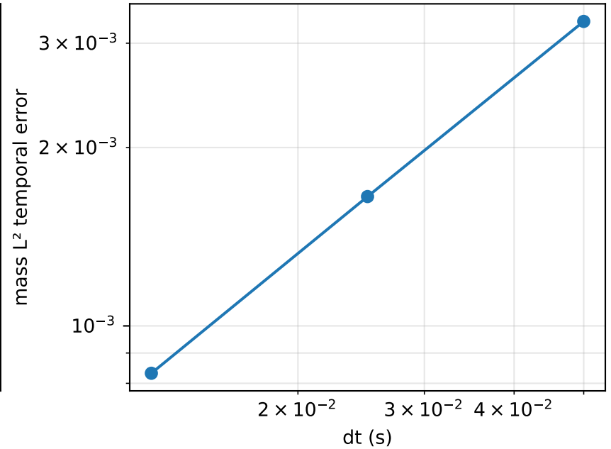
Dense ALE reference: first-order time error
