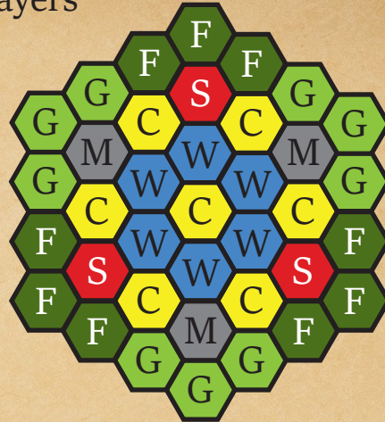
3 Players
