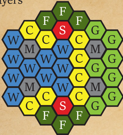
2 Players
