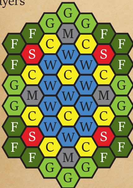
4 Players
