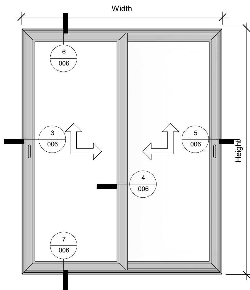
1 Elevation Front 1 : 20
