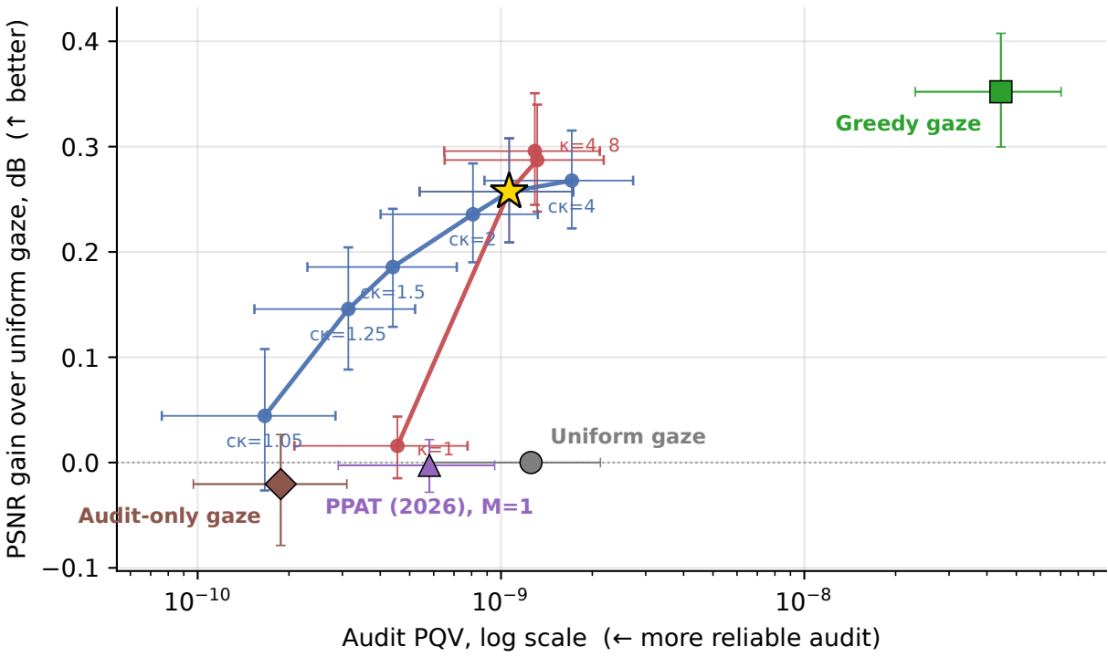
REDS val (15 clips)
