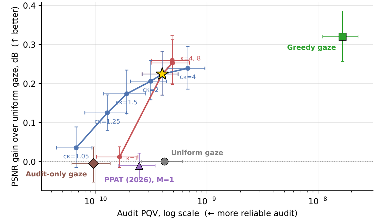
REDS train (15 clips)
