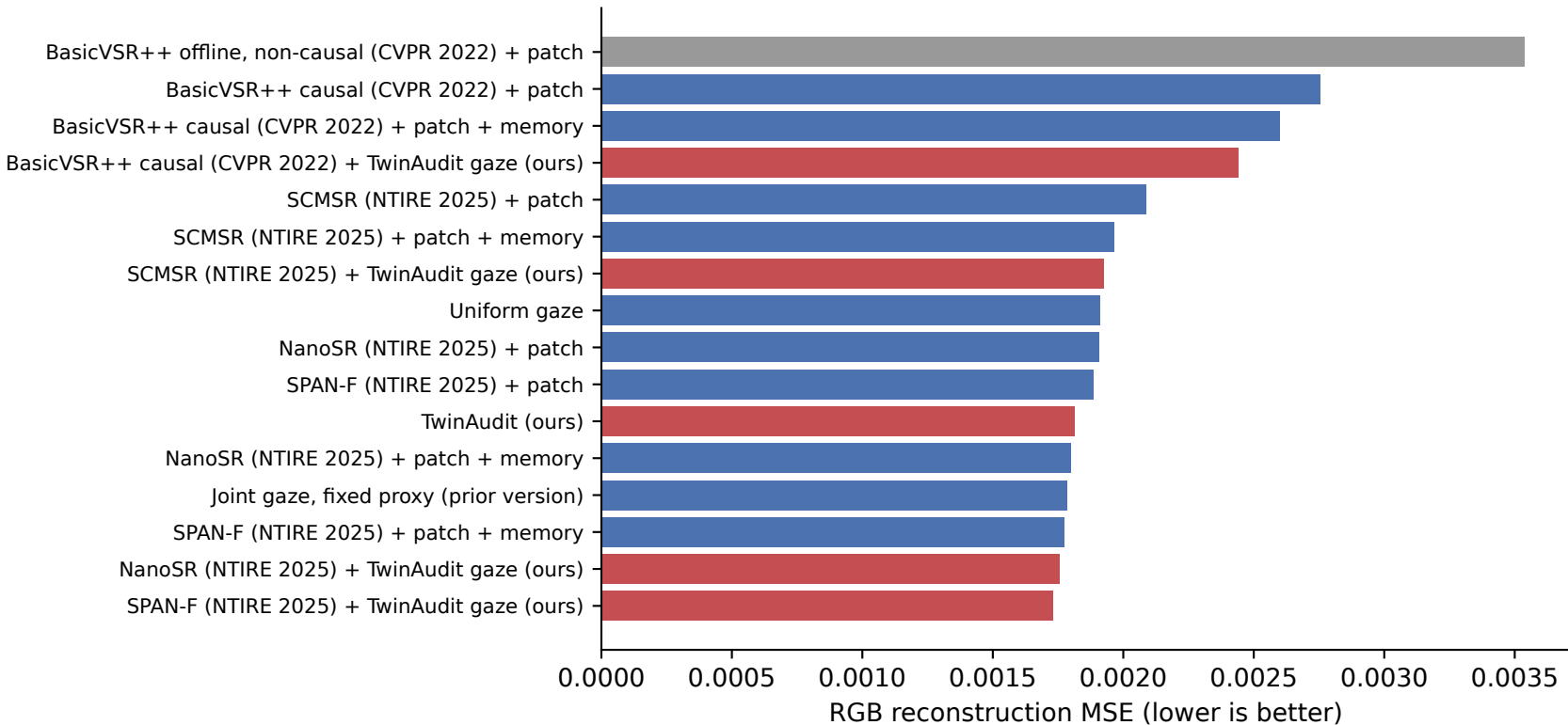
DAVIS - sensor-noise input
