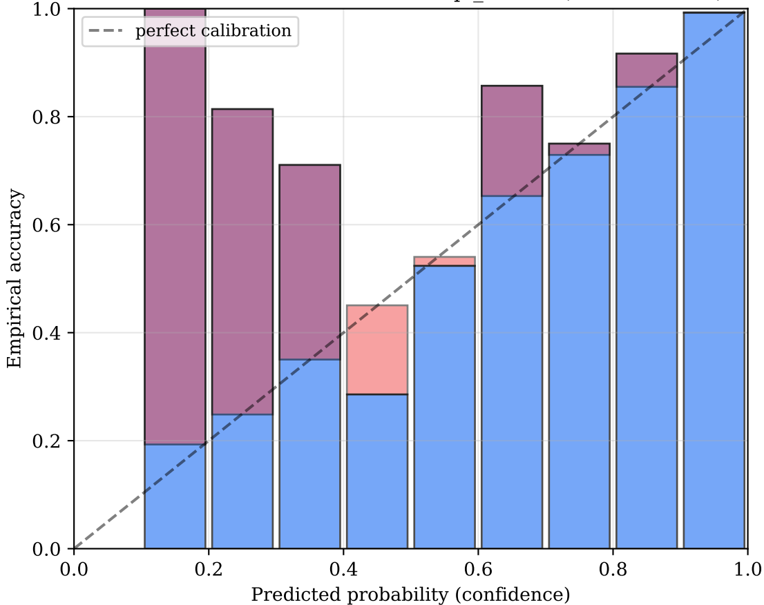
Calibration — herbert/finetune on pl_claims (ECE = 0.1082)
