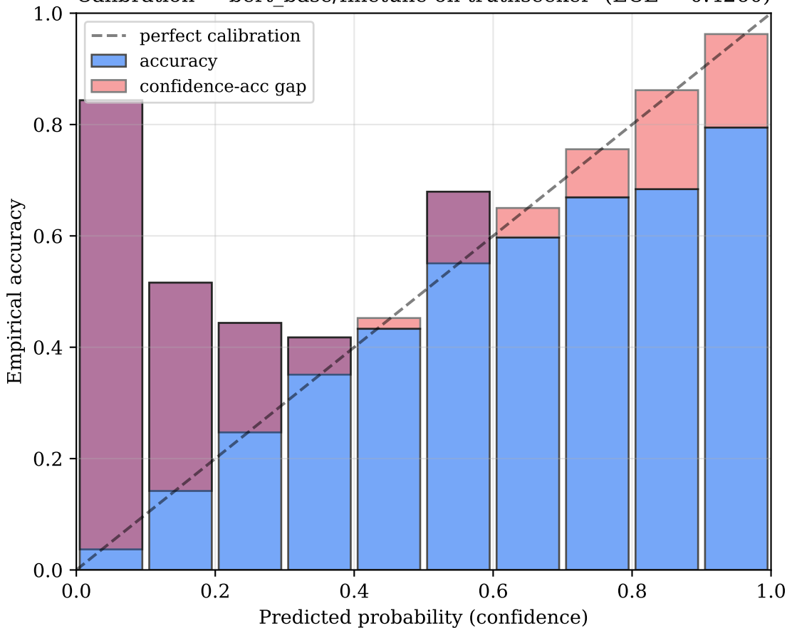
Calibration — bert_base/finetune on truthseeker (ECE = 0.4260)
