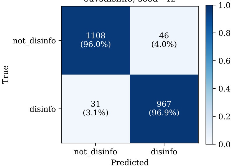
CM — mbert/finetune euvsdisinfo, seed=42
