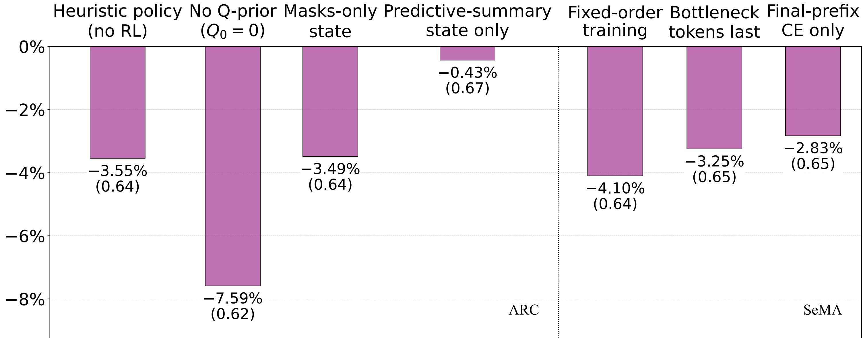
Relative Macro-F1 change (%)
