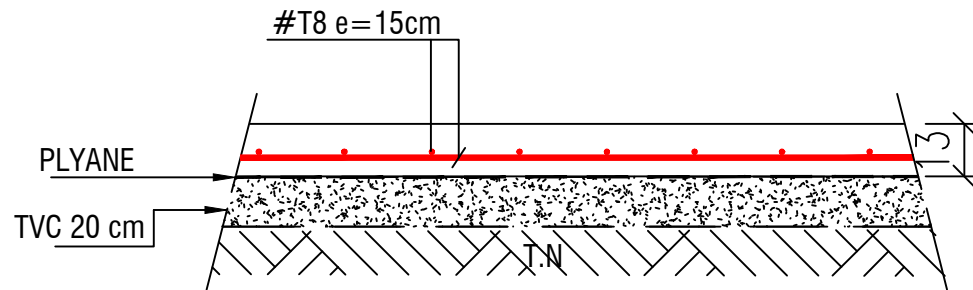
DALLAGE TYPE13
