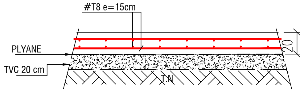
DALLAGE TYPE20
