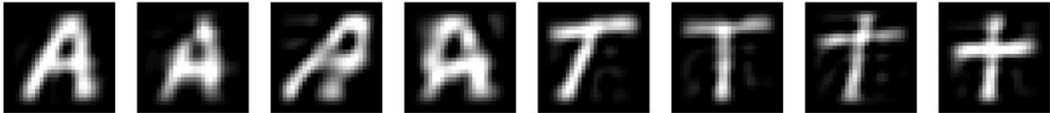
Certificate (native Levenberg-Marquardt)
