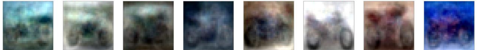
recovered residual 3e-29
